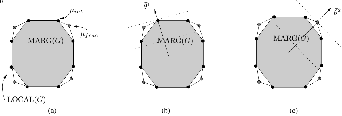
Fig. 2. (a) The constraint set LOCAL(G) is an outer bound on the exact marginal polytope. Its vertex set includes all the integral vertices of MARG(G) , which are in one-to-one correspondence with optimal solutions of the integer program. It also includes additional fractional vertices, which are not vertices of MARG(G) . (b)–(c) Solving a LP with cost vector \bar{\theta} entails translating a hyperplane with normal \bar{\theta} until it is tangent to the constraint set LOCAL(G) . In (b), the point of tangency occurs at a unique integral vertex. In (c), the tangency occurs at a fractional vertex of LOCAL(G) that lies outside of MARG(G) .
