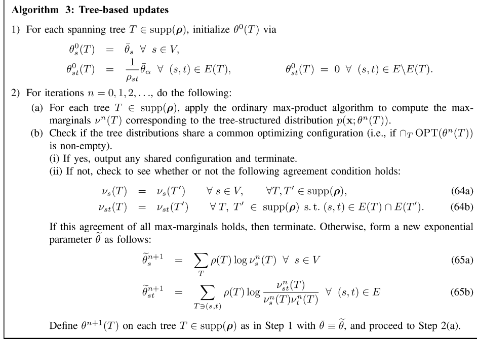
Fig. 7. Tree-based updates for finding a tree-consistent set of pseudo-max-marginals.
