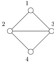
Fig. 5. Simple diamond graph G_{\text{dia}} .
