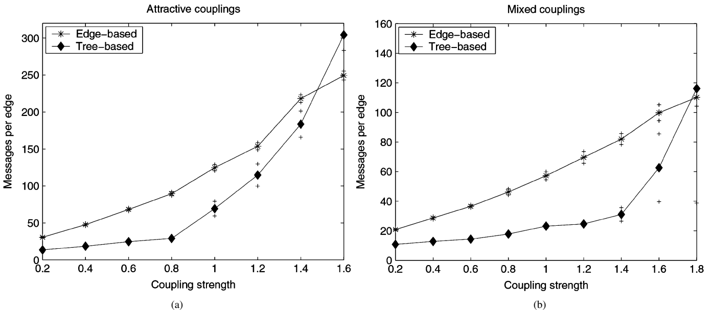
Fig. 6. Comparison of parallel edge-based message-passing (Algorithm 2) and tree-based updates (Algorithm 3 described in the Appendix, part C) on a nearest neighbor grid with n = 400 variables. (a) Attractive couplings. (b) Mixed couplings.
