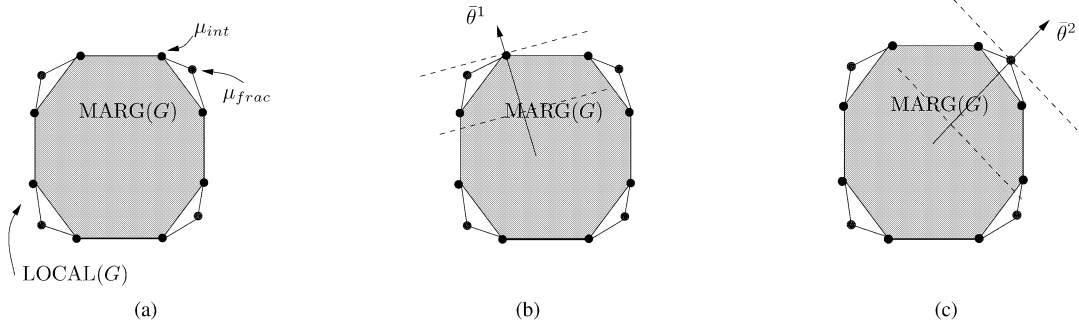
Fig. 2. (a) The constraint set LOCAL(G) is an outer bound on the exact marginal polytope. Its vertex set includes all the integral vertices of MARG(G) , which are in one-to-one correspondence with optimal solutions of the integer program. It also includes additional fractional vertices, which are not vertices of MARG(G) . (b), (c) Solving an LP with cost vector \bar{\theta} entails translating a hyperplane with normal \bar{\theta} until it is tangent to the constraint set LOCAL(G) . In (b), the point of tangency occurs at a unique integral vertex. In (c), the tangency occurs at a fractional vertex of LOCAL(G) that lies outside of MARG(G) .
