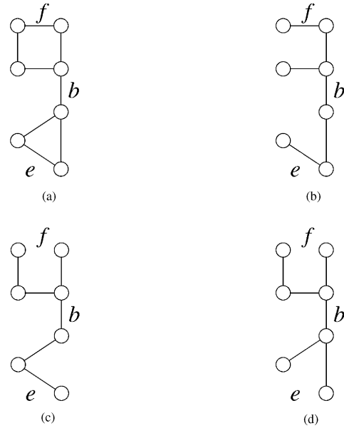
Fig. 1. Illustration of edge appearance probabilities. Original graph is shown in panel (a). Probability 1/3 is assigned to each of the three spanning trees \{T_i \mid i = 1, 2, 3\} is shown in panels (b)–(d). Edge b is a so-called bridge in G , meaning that it must appear in any spanning tree. Therefore, it has edge appearance probability \rho_b = 1 . Edges e and f appear in two and one of the spanning trees, respectively, which gives rise to edge appearance probabilities \rho_e = 2/3 and \rho_f = 1/3 .
