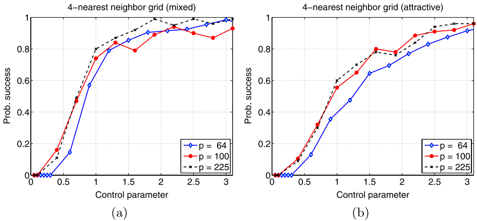
FIG. 2. Plots of success probability \mathbb{P}[\widehat{\mathcal{N}}_{\pm}(r) = \mathcal{N}(r), \forall r] versus the control parameter \beta(n, p, d) = n / [10d \log(p)] for Ising models on 2-D grids with four nearest-neighbor interactions ( d = 4 ). (a) Randomly chosen mixed sign couplings \theta_{st}^* = \pm 0.50 . (b) All positive couplings \theta_{st}^* = 0.50 .
