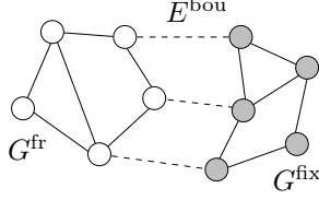
Figure 1. Partition of the graph G into a subgraph G^{\text{fix}} = G[V^{\text{fix}}] induced by the fixed vertices, and a subgraph G^{\text{fr}} = G[V^{\text{fr}}] induced by free vertices. The boundary edges E^{\text{bou}} cross between these two node-induced subgraphs.
