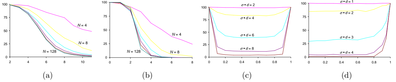
Figure 2. Panels (a) and (b): Plots of correct percentage p_{\text{cor}} versus the potential strength \sigma \cdot d (where \sigma is interaction strength and d is node degree) for grids (panel (a)) and complete graphs (panel (b)). Different curves in each panel correspond to different graph sizes N \in \{4, 8, 16, 32, 64, 128\} (from top to bottom). Panels (c) and (d): Plots of correct percentage p_{\text{cor}} versus the mixing parameter \alpha \in [0, 1] for grids (panel (c)) complete graphs (panel (d)). Different curves in each panel correspond to different potential strengths \sigma \cdot d \in \{2, 4, 6, 8, 10\} for grids and \sigma \cdot d \in \{1, 2, 3, 4, 5\} for complete graphs (from top to bottom).
