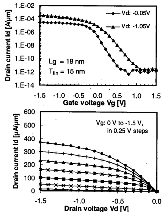
Figure 5: IV characteristics of PMOS FinFET with 18-nm gate length and 15-nm Si fin body.
