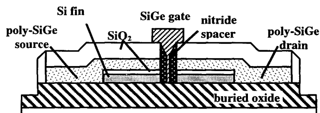
Figure 1: Schematic drawing of FinFET
