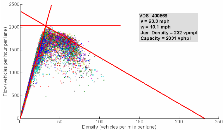
FIGURE 3. The last result of the calibration with the regression line for the congestion parameter, w , and values for the calibrated parameters.
