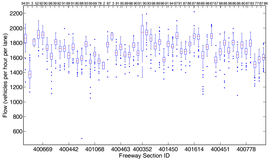
FIGURE 4. Boxplots showing the variation in capacity of successive freeway sections among many days.
