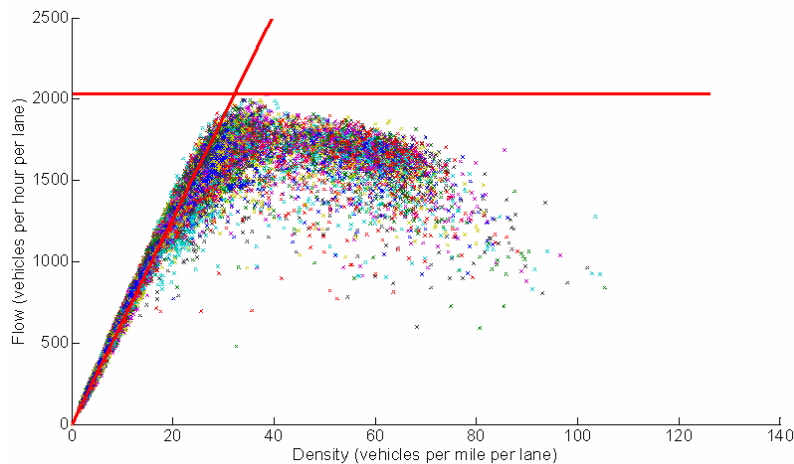
FIGURE 2. The estimation of free-flow speed and capacity.
