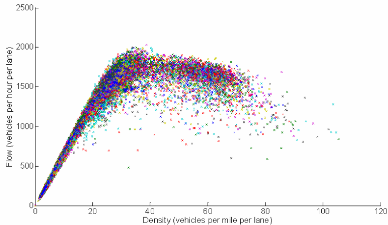
FIGURE 1. Flow vs Density scatter plot of vds 400669 on I-880 Southbound accumulated over 92 days' data. Each dot on the plot corresponds to one observed flow – density pair. Each day has 288 such data points.
