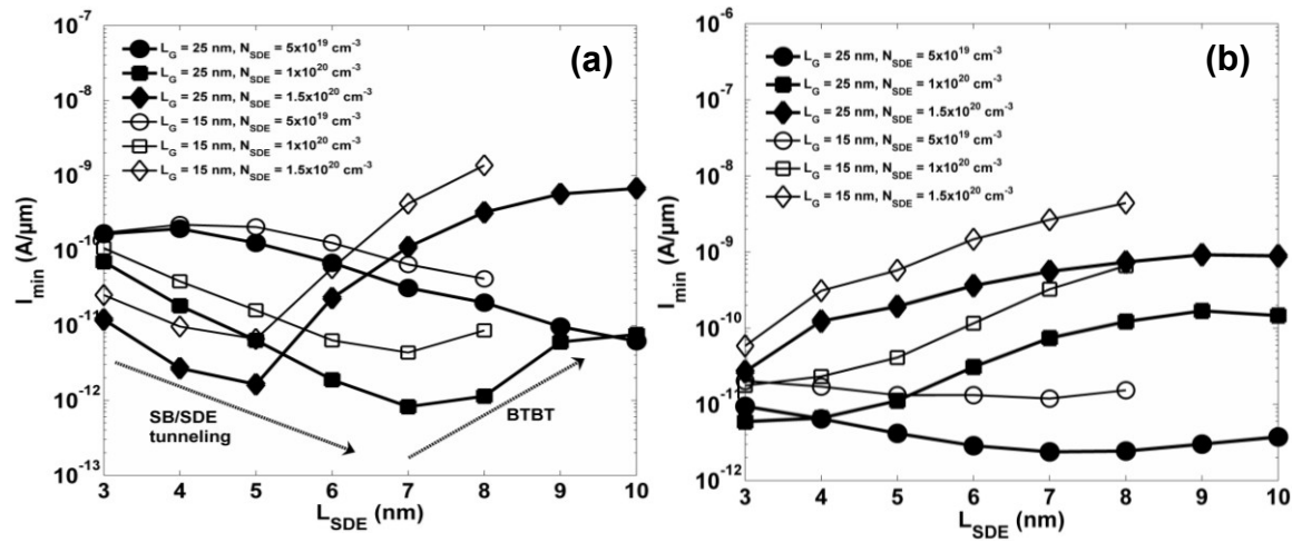
Fig. 2.7. I_{min} vs. L_{SDE} for SDG FETs with (a) \text{NiSi} and (b) \text{ErSi}_{1.7} MSD regions, and N_{SDE} = 5 \times 10^{19} - 1.5 \times 10^{20} \text{ cm}^{-3} . EOT = 1 \text{ nm} , t_{body} = 10 \text{ nm} , L_{un} = 8 \text{ nm} , and V_{DS} = 1 \text{ V} .
