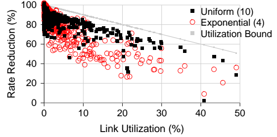
Figure 12: Rate reduction per link
