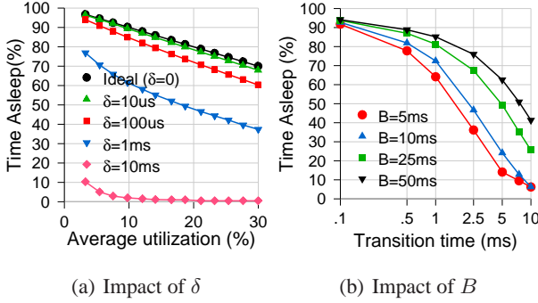
Figure 6: The impact of hardware constants on sleep time.
