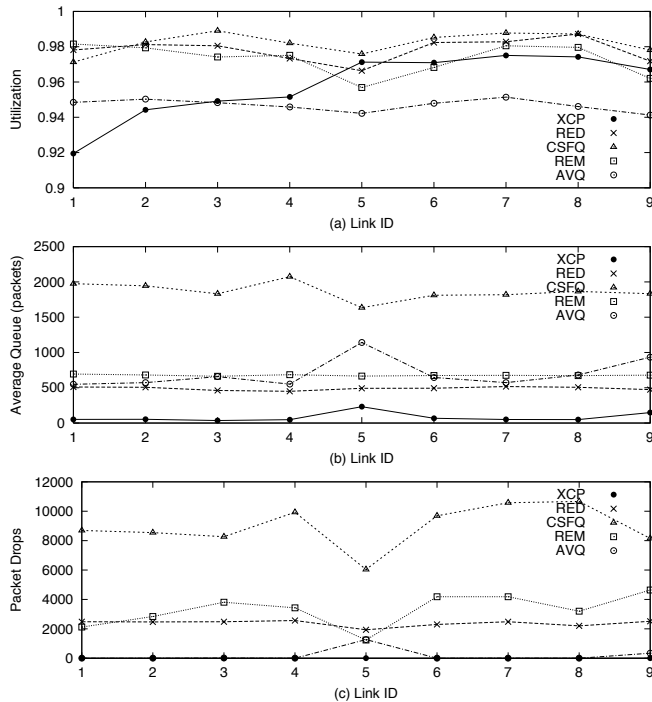
Figure 11: Simulation with multiple congested queues. Utilization, average Queue size, and number of drops at nine consecutive links (topology in Figure 3). Link 5 has the lowest capacity along the path.
