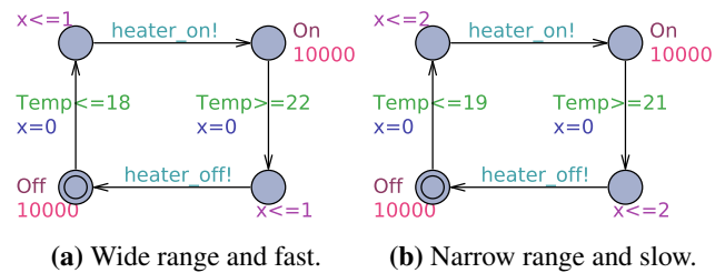
Figure 10. Stochastic controllers use regular (non-urgent) channels, therefore timings are stochastic: delays are distributed uniformly (when clock invariant is used) and exponentially (in locations On and Off ).
