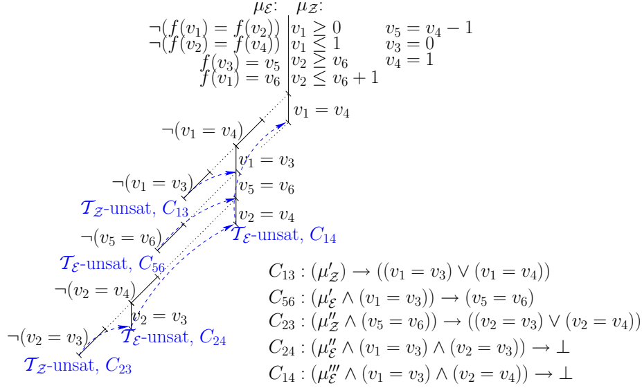
Figure 12.6. The DTC search tree for Example 12.6.3 on \mathcal{T}_{\mathcal{Z}} \cup \mathcal{T}_{\mathcal{E}} , with no e_{ij} -deduction. v_1, \dots, v_6 are interface terms. \mu'_{\mathcal{T}_i}, \mu''_{\mathcal{T}_i}, \mu'''_{\mathcal{T}_i} denote appropriate subsets of \mu_{\mathcal{T}_i} , \mathcal{T}_i \in \{\mathcal{T}_{\mathcal{E}}, \mathcal{T}_{\mathcal{Z}}\} .
