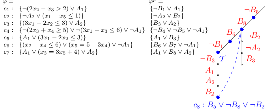
Figure 12.4. Boolean search (sub)tree in the scenario of Example 12.4.1. (A diagonal line, a vertical line and a vertical line tagged with “ \mathcal{T} ” denote literal selection, unit propagation and \mathcal{T} -propagation respectively; a bullet “ \bullet ” denotes a call to the \mathcal{T} -solver.)
