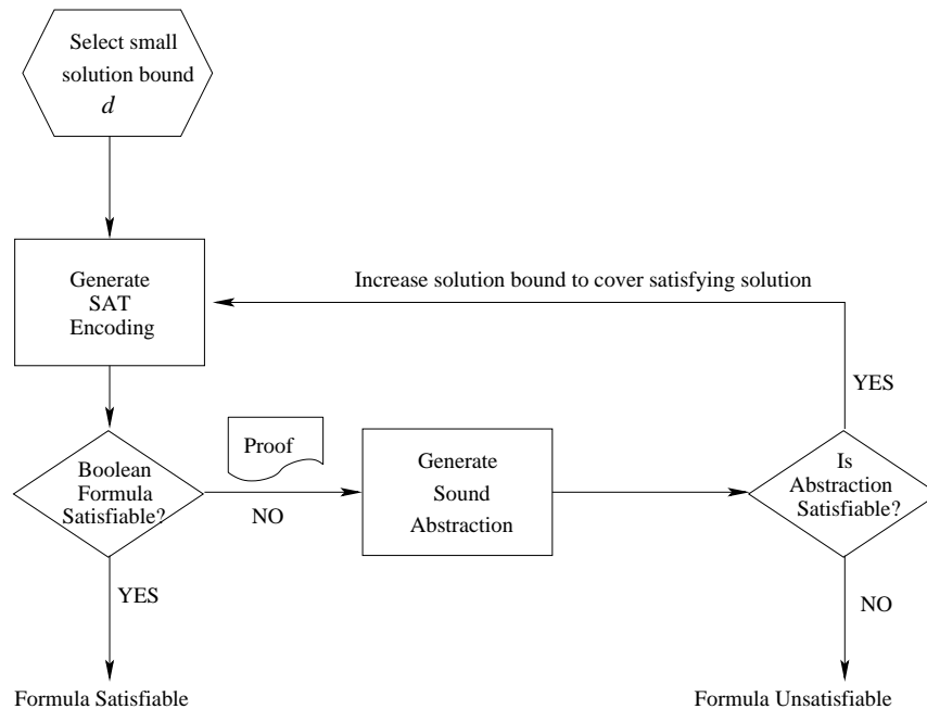
Figure 12.7. Lazy approach to computing solution bound
