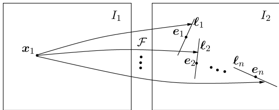
Figure 3. The multibody fundamental matrix \mathcal{F} maps each point \mathbf{x}_1 in the first image to n epipolar lines \ell_1, \dots, \ell_n which pass through the n epipoles e_1, \dots, e_n respectively. One of these epipolar lines must pass through \mathbf{x}_2 .
