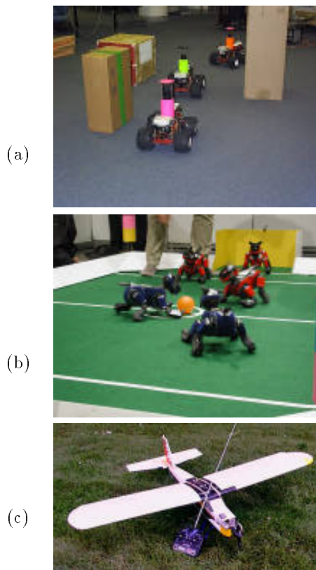
Figure 14: The GRASP/UPenn multi-vehicle testbed includes (a) seven wheeled platforms equipped with omnidirectional cameras; (b) legged robots with visual sensing; and (c) three UAVs, including quadrotor helicopters with cameras for indoor operation (not shown).
