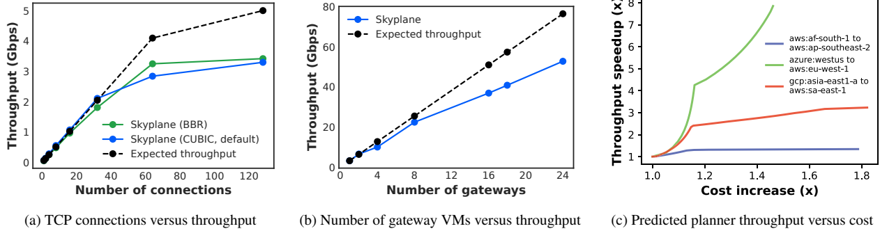
Figure 9: Skyplane ablations: We evaluate the impact of parallel TCP connections, parallel gateway VMs and overlay cost.
