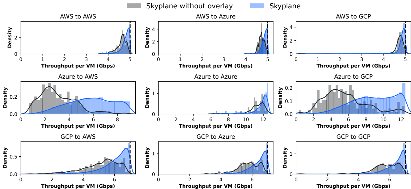
Figure 7: Ablation of predicted overlays: Overlay routes improve throughput per VM instance. We visualize the distribution of predicted throughput by the planner with all optimizations enabled (Skyplane) and with all optimizations except for overlay routing (Skyplane without overlay). The AWS and GCP egress limits are displayed with a dashed line.
