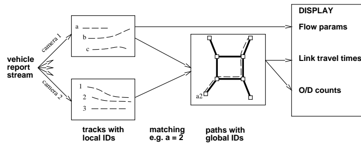
Fig. 2. Overall design of our traffic surveillance system. The video streams are processed at each camera site by vehicle tracking software running on customized parallel hardware. The resulting streams of chronologically ordered vehicle reports are sent to the TMC (Traffic Management Center). The TMC uses these reports to determine when a vehicle detected at one camera has reappeared at another. These matches are used to build up a path for each vehicle as it travels through the freeway network. The set of paths can be queried to compute link travel times and O/D counts as desired. The output of the system is a traffic information display, updated in real time for use by traffic operations managers or by individual drivers.
