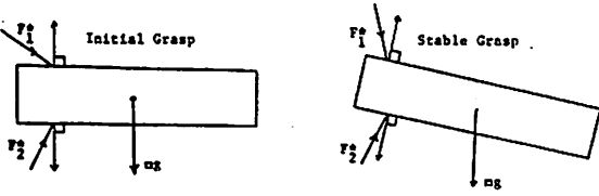
Figure 11. Grasping with Gravitational Force
