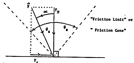
Figure 1. Friction Principles
