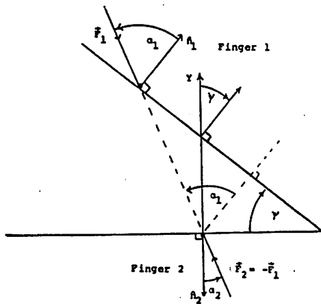
Figure 2. Angles of Force for Polygon in Equilibrium
