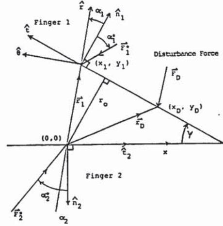
Figure 10. Grasping with Disturbance Forces
