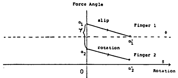
Figure 8. Rotation During Hand Priority Grasp
