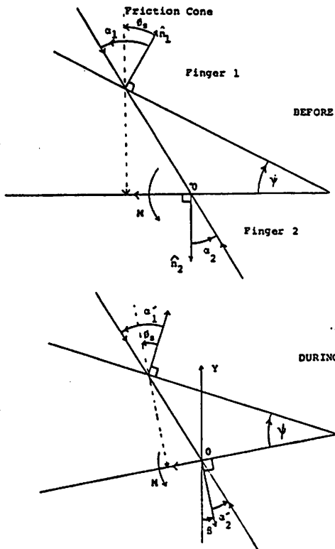
Figure 7. Hand Priority Grasp
