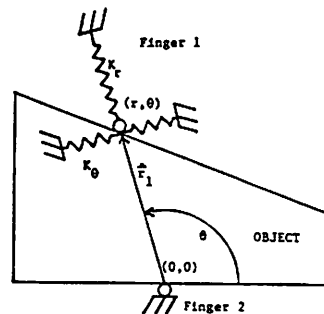
Figure 6. Polar Stiffness Representation
