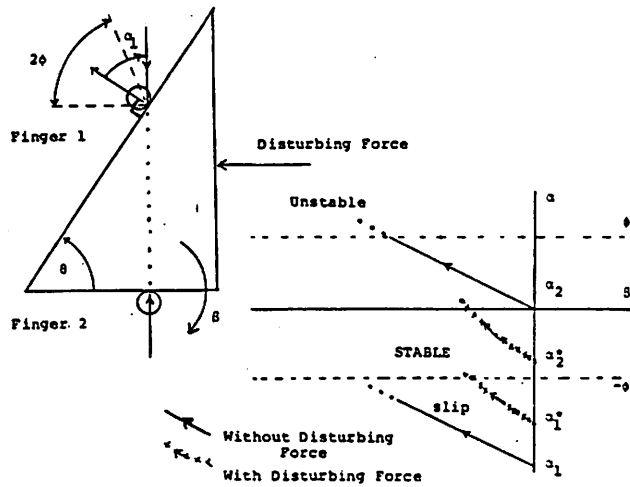
Figure 13. Making a Grasp Stable
