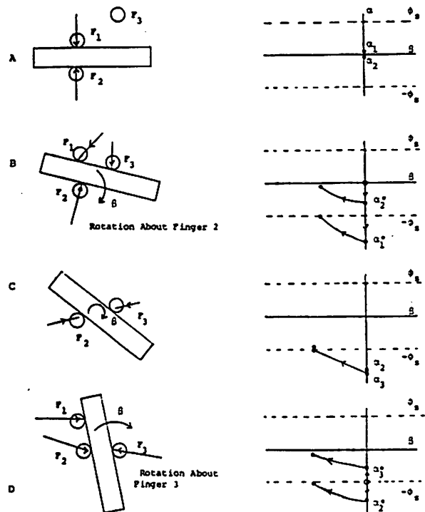
Figure 14. "Classical" Reorientation/Regrasp Example
