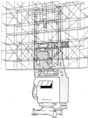
FIG. 7.3 Freya Working at about 125 MHz and rotating through 3 degrees, Freya was the main German surveillance radar throughout the Second World War, deployed for both coastal and inland surveillance.
