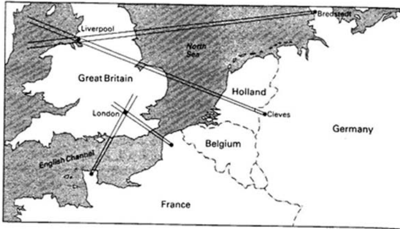
FIG. 9.1 Knickebein Germany's first navigational and targeting system
