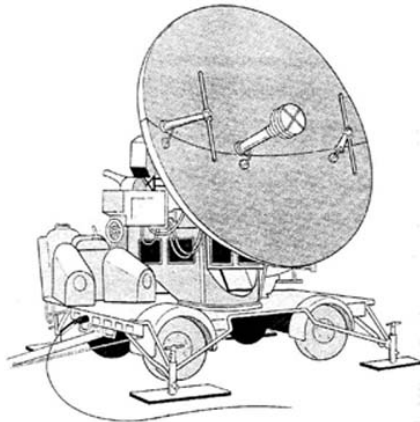
FIG. 8.2 Wurzburg Wurzburg was primarily a target-tracking radar, combining a parabolic antenna with a central rotating dipole to obtain conical scanning. It provided accurate azimuth and elevation. Frequency was about 560 MHz. The vertical rods are secondary radar (identification friend or foe (IFF)) antennas.
