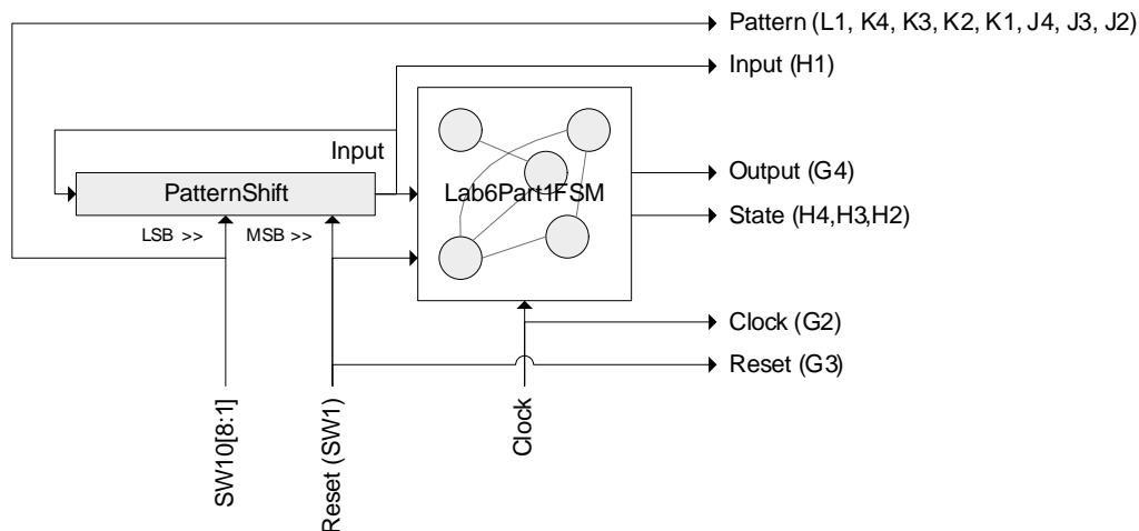
Figure 1: Lab #5 Part 1 Test Harness
