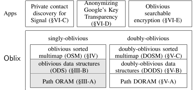
Figure 1: Component stack of Oblix. Grey blocks are components that exist before Oblix, and white blocks are Oblix’s contributions.
