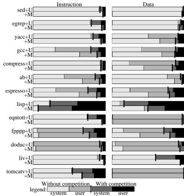
Figure 4-1: User/system interference.
