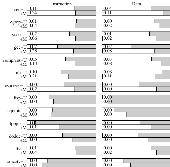
Figure 4-2: System self-interference.
