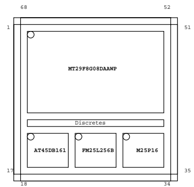
Figure 1: System PCB floorplan.
