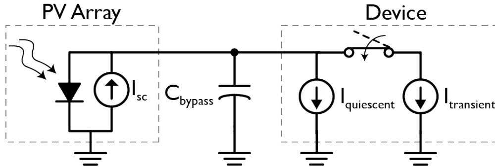
Figure 2.1: Model used to maintain proper operating voltages and functionality of SARA. Typically I_{quiescent}=350 \mu\text{A} and I_{transient}=1250 \mu\text{A} during radio operation.
