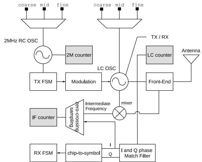
Fig. 2. Interconnection between the on-chip oscillators, counters, and the related radio components of SC\mu M .
