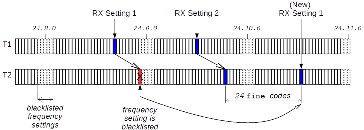
Fig. 8. We blacklist all frequency settings in ranges (\text{coarse.mid}, 30) and (\text{coarse.mid}+1, 2) . At time T1 , the radio hops between RX frequency settings (24.8.22) and (24.9.16) . Frequency trimming is used on both independently; at time T2 , trimming causes the settings to evolve to (24.8.30) and (24.9.25) . Since setting (24.8.30) falls in the blacklisted settings, it is replaced by a setting 24 fine code above the other setting, i.e., (24.10.17) .
