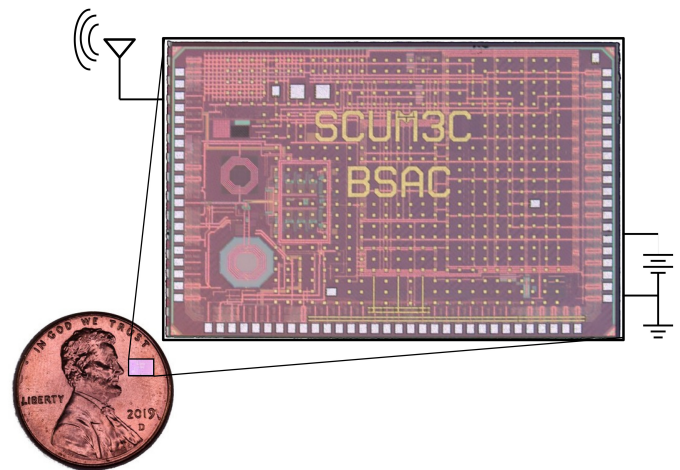
Fig. 1. SC \mu M is a 2×3 mm 2 crystal-free mote-on-chip. It functions without any external components other than a power source and an antenna, and implements the IEEE802.15.4 [2] and BLE standards.
