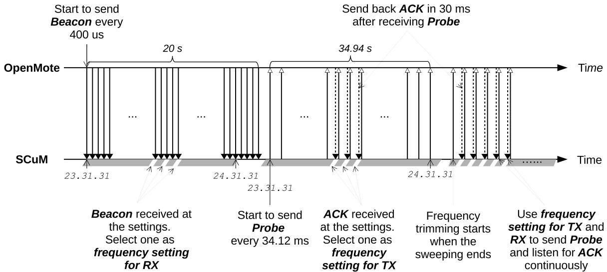
Fig. 6. Frequency sweep step of CoCa. The OpenMote sends a burst of Beacon frames on a single frequency, one every 400 \mu s. SC \mu M sweeps its 2.4-GHz LC frequency settings from (23.31.31) to (24.31.31), listening for Beacon frames. It records the best setting on which it receives Beacon frames as its RX frequency setting. After sending the burst of Beacon frames, the OpenMote continuously listens for Probe frames; it sends back an ACK frame if it receives one. SC \mu M does a second sweep through its frequency settings, this time sending a Probe frame for each setting and listening for an ACK frame. It records the “best setting” (detailed in [20]) on which it transmitted a Probe frame it received an ACK for, as its frequency setting for transmitting (TX). After this, the frequency trimming step (Section V-D) starts.
