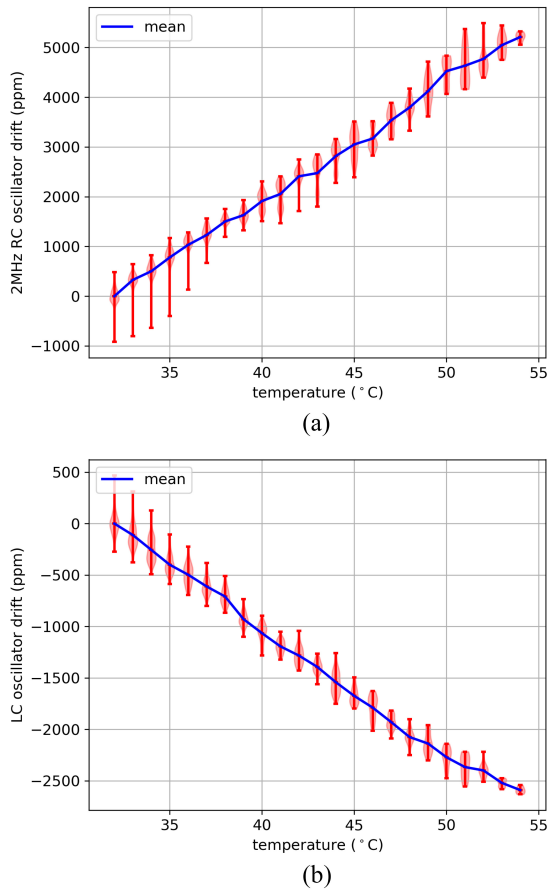
Fig. 4. Evolution of the frequency of the 2-MHz RC oscillator and the 2.4-GHz LC oscillator over a 30–55 °C temperature range, when tuned statically to (22.17.15) and (24.10.22), respectively. (a) 2-MHz RC oscillator. (b) 2.4-GHz LC oscillator (RX).
