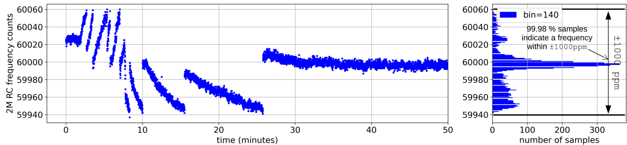
Fig. 15. 2-MHz count evolving over time ( left ) and the corresponding distribution ( right ). 99.98% of the measurements fall within the \pm 1000 ppm range mandated by the IEEE802.15.4 standard.
