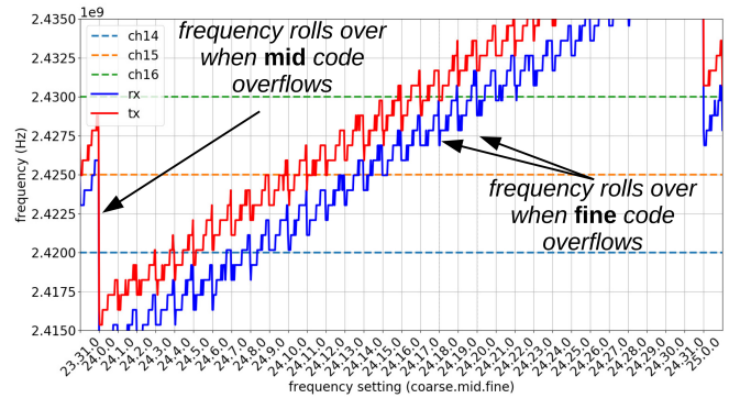
Fig. 3. LC frequency as a function of the frequency setting, for values from (23.31.0) to (25.0.31). While the frequency increases with the frequency setting, the frequency drops when the fine or mid codes overflow, resulting in a nonlinear saw-tooth shape.
