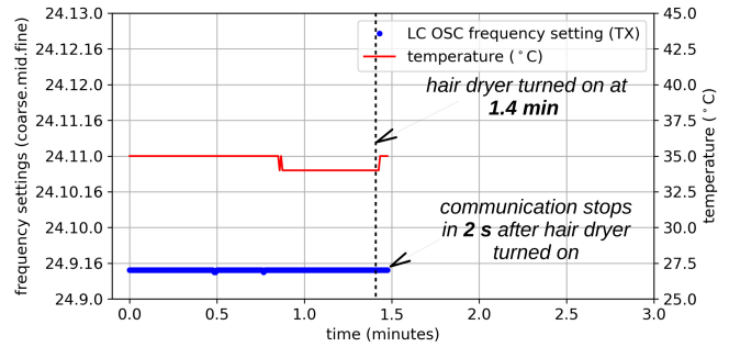
Fig. 5. Showing communication fail when SCμM does not continuously calibrate its oscillators. We precalibrate SCμM to it is able to communicate with an OpenMote. Each (blue) dot indicates successful communication. After about a minutes, when turn on a hair dryer pointed at SCμM. Less than 2 s after turning on the hair dryer, communication stops. As an artefact of how the experiment is done, the temperature stops being reported when communication stops.
