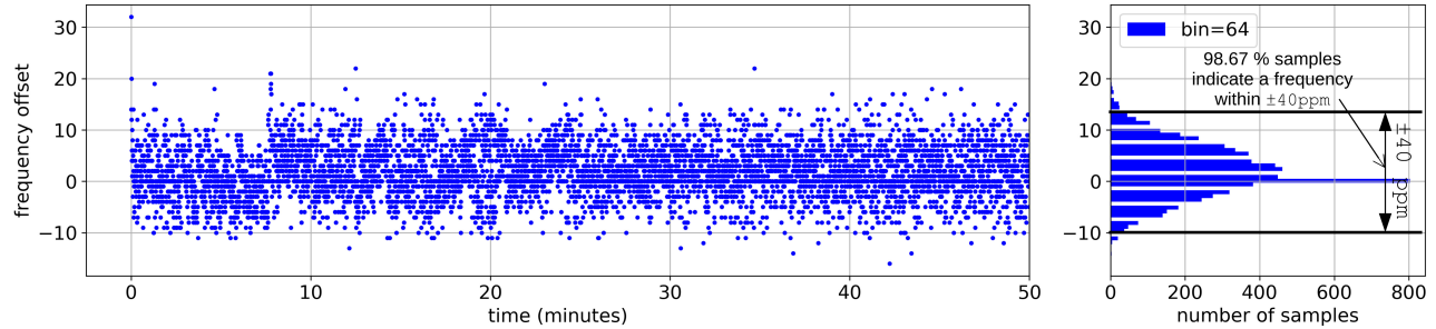
Fig. 14. FO evolving over time ( left ) and the corresponding distribution ( right ). 98.67% of the measurements fall within the \pm 40 ppm range mandated by the IEEE802.15.4 standard.
