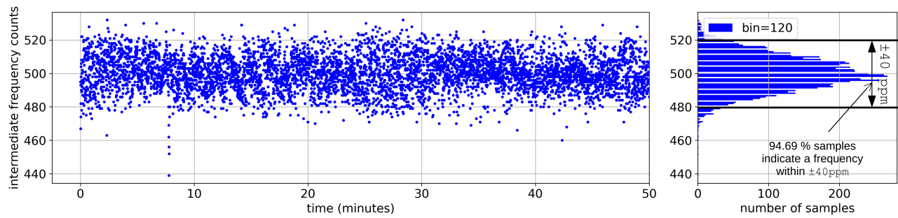
Fig. 13. Number of IF zero-crossings over time ( left ) and the corresponding distribution ( right ). 94.69% of the measurements fall within the \pm 40 ppm range mandated by the IEEE802.15.4 standard.
