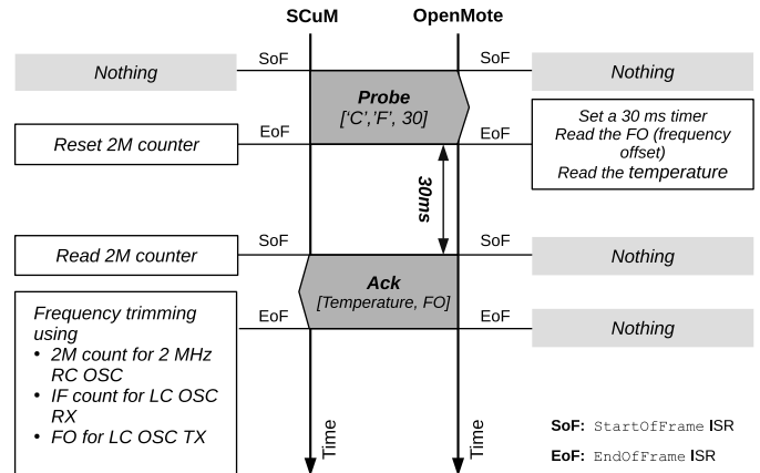
Fig. 7. SC \mu M resets its 2-MHz RC counter when it just finished transmitting the Probe frame. Upon receiving a Probe frame, OpenMote records its FO (read from its FREEST register). It then waits exactly 30 ms, before sending an ACK frame containing the FO. Upon receiving ACK frame, SC \mu M reads the value of its 2-MHz RC counter to calibrate it 2-MHz RC oscillator setting, uses the FO value to calibrate its 2.4-GHz LC oscillator setting in the TX mode, and measures the number of zero-crossing to calibrate its 2.4-GHz LC oscillator setting in the RX mode.
