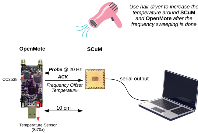
Fig. 9. SC \mu M sends Probe frames to OpenMote, one every 50 ms. The OpenMote sends back an ACK frame that contains the FO and the temperature. We use a hairdryer to increase the temperature of SC \mu M. We place an OpenMote board only 10-cm away from SC \mu M, and point the hair dryer at both. This allows us to measure the temperature at SC \mu M.
