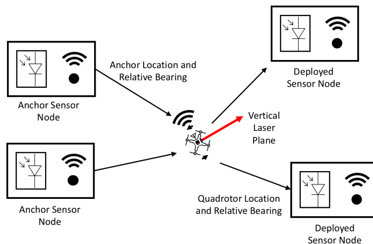
Figure 1. Schematic of proposed distributed lighthouse self-localization. The quadrotor can act as a lighthouse base station by rotating in order to obtain relative bearings between itself and wireless sensor nodes with known locations, or anchor sensor nodes . In this system, the quadrotor can localize itself based on bearing measurements relative to these anchor sensor nodes. The quadrotor can also provide relative bearing measurements to recently deployed sensor nodes with unknown locations ( deployed sensor nodes ), which allows them to localize themselves.
