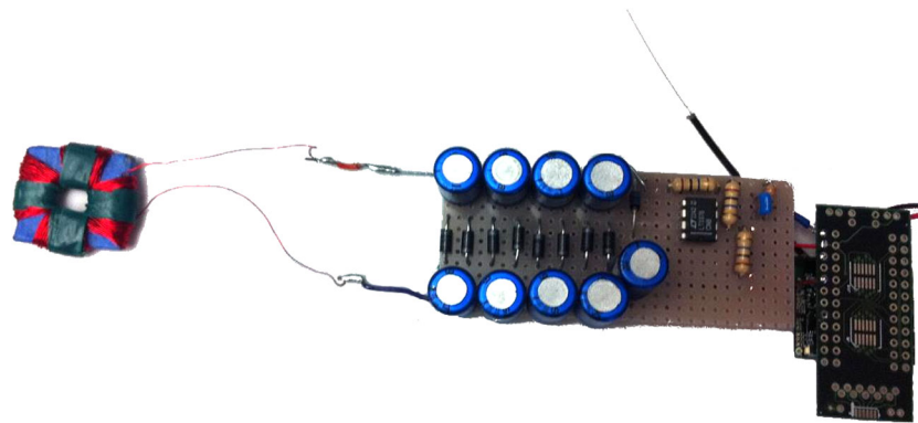
Figure 11. Guidance Inertial and Navigation Assistant platform connected to a contact-less (plug-through) power-line energy scavenger and consuming 68 \mu\text{A} average. It uses OpenWSN and Constrained Application Protocol to report current usage every 2 s to a server on the Internet.
