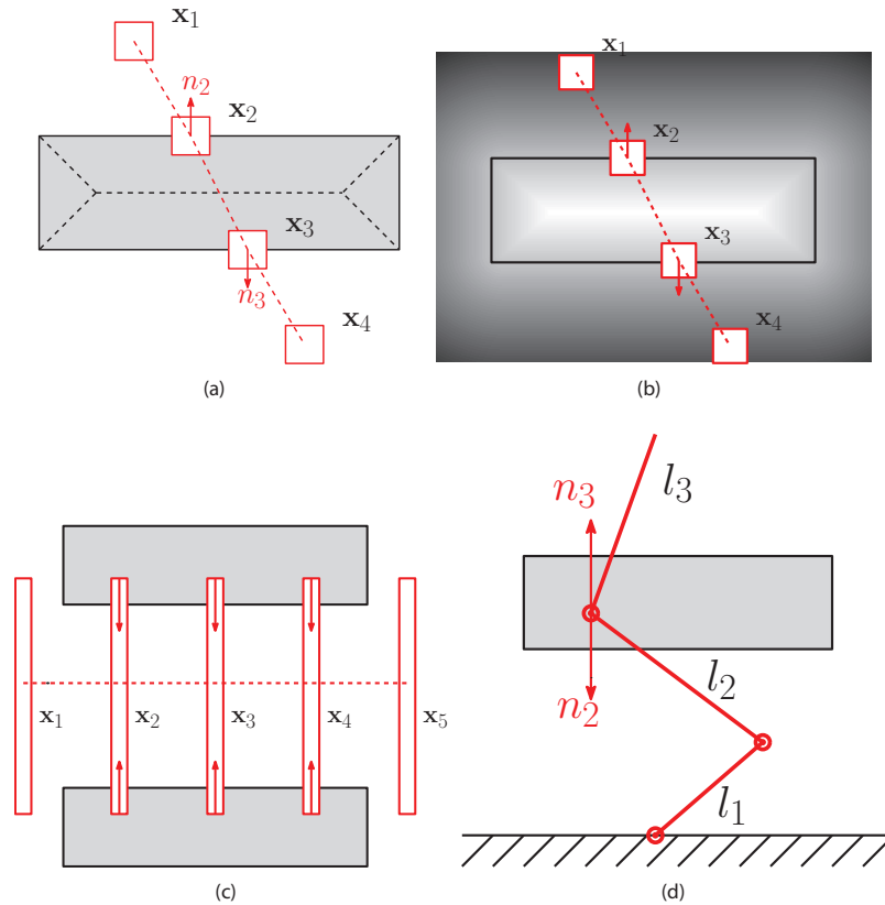
Fig. 13. Illustration of typical reasons for trajectory optimization to get stuck in local optima that are not collision-free. (a) The gradient based on penetration depth may push waypoints in inconsistent directions. (b) The gradient based on distance fields has the same problem. (c) When a robot collides simultaneously with multiple obstacles, the robot may get stuck in an infeasible local optimum as different obstacles push the robot in different directions. (d) For a robot with multiple links, the gradient may result in inconsistent directions for different links. x_i in these figures denote configurations at different time steps along the trajectory.
