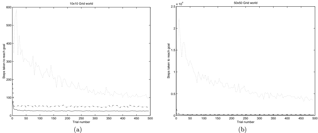
Figure 1: (a) Experiment with 10x10 grid-world. Plot of steps taken to goal vs. trial number. Dot is no shaping, dot-dash is \Phi = 0.5\Phi_0 , solid is \Phi = \Phi_0 . (b) Experiment with 50x50 grid-world.
