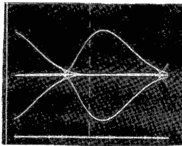
Transmitted pulse shape 200mV/cm 2 \mu s/cm (a)
