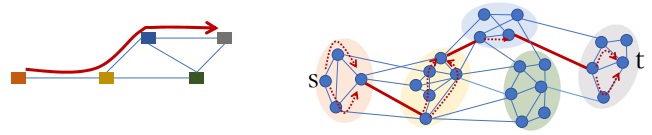
Figure 10: Contrasting with Figure 9, for the same cluster bundle, in a subsequent iteration, NCFLOW allocates flow on a different path on the aggregate graph and on different inter-cluster edges. The chosen paths and edges are again shown in red.
