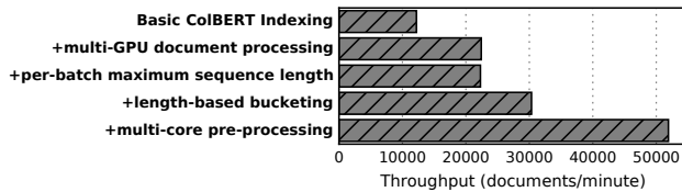
Figure 6: Effect of ColBERT’s indexing optimizations on the offline indexing throughput.
