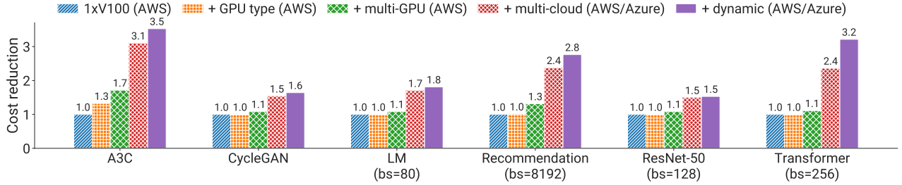
Figure 5: Average cost reduction to run the same number of training iterations (4 V100-days of computation), while cumulatively adding more sources of price variation. 1xV100 uses the cheapest 1xV100 instance within the us-east-1 AWS region, GPU type chooses the GPU with highest cost-normalized throughput, multi-GPU picks instances with multiple GPUs if they are cheaper on a per-GPU basis; all these strategies use AWS instances only. The multi-cloud strategy picks the cheapest instance across AWS and Azure at the start of training, and then sticks with this choice throughout training. Dynamic continually picks the cheapest instance across AWS and Azure through training as prices change. Costs reduce as sources of price variation are added.
