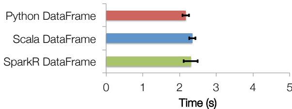
Figure 4: SparkR Performance Comparison with Python, Scala APIs
