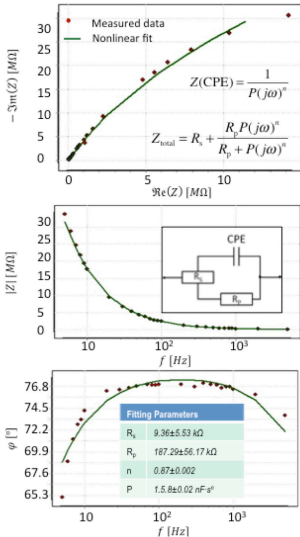
Fig. 5. Characterization of the electrode-electrolyte interface by electrochemical impedance spectroscopy.
