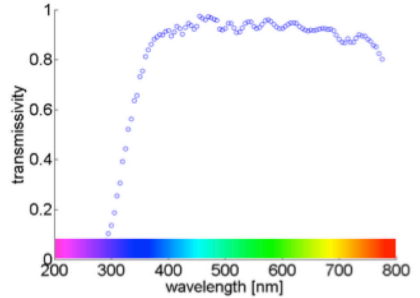
Fig. 4. The optical transmissivity of the 110 nm thin ITO film exceeds 90% over most of the visible spectrum.
