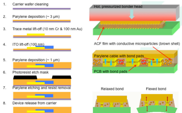
Fig. 2. Fabrication and Assembly. Left: Au-ITO hybrid device fabrication process. Top right: The ACF film is thermo-compressed between complementary pad arrays. Top middle: Au-coated polymer microspheres embedded in the epoxy establish a robust electrical connection. Between adjacent pads the microparticles remain surrounded by insulating polymer that prevents shorts. Bottom right: The cured epoxy provides mechanical stability under flexion. Image sources: ITO America Corp. and Tatsuo Nagamatsu, 12th Annual KGD Packaging and Test Workshop, Sept. 12-15 2005, Napa, CA (recolored).
