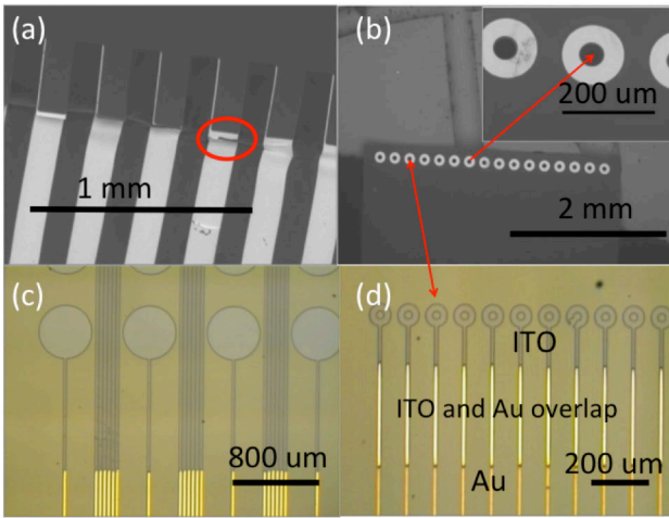
Fig. 3. Micrographs and SEM images of the 16-channel and 49-channel devices. (a) Bond pad damage on ITO-only devices. (b) Intact electrodes of a 16-channel ITO device. (c) Electrodes and interconnects of a 49-channel Au-ITO hybrid device. (d) 16-channel hybrid array. The ring-shaped electrodes are made of ITO. The light yellow lines indicate the overlap of Au and ITO. The lower part of the connections consists of Cr/Au.
