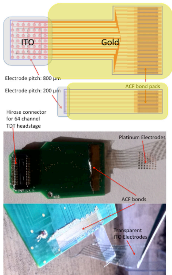
Fig. 1. Top: ECoG CAD designs (49 channel 2D array with 800 \mu\text{m} pitch and 16 channel linear array with 200 \mu\text{m} pitch). Bottom left: Baseline (Cr/Au/Pt stack) ECoG. Bottom right: Hybrid Au-ITO ECoG.
