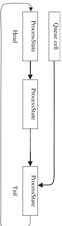
Figure 1: A process queue
