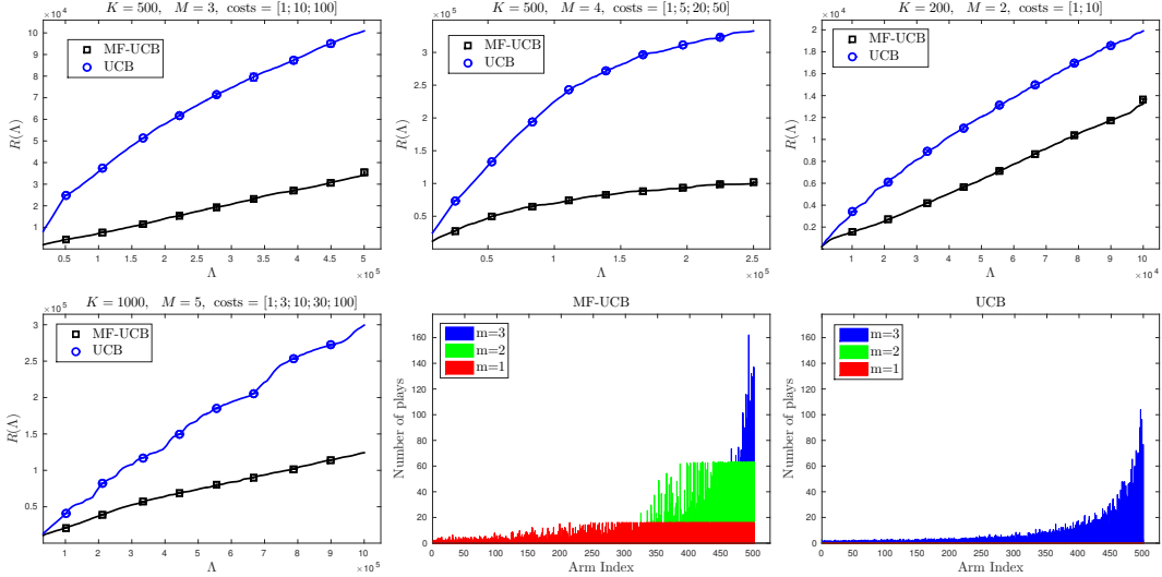
Figure 2: Simulations results on the synthetic problems. The first four figures compares UCB against MF-UCB on four synthetic problems. The title states K, M and the costs \lambda^{(1)}, \dots, \lambda^{(M)} . The first two used Gaussian rewards and the last two used Bernoulli rewards. The last two figures show the number of plays by UCB and MF-UCB on a K = 500, M = 3 problem with Gaussian observations (corresponding to the first figure).
