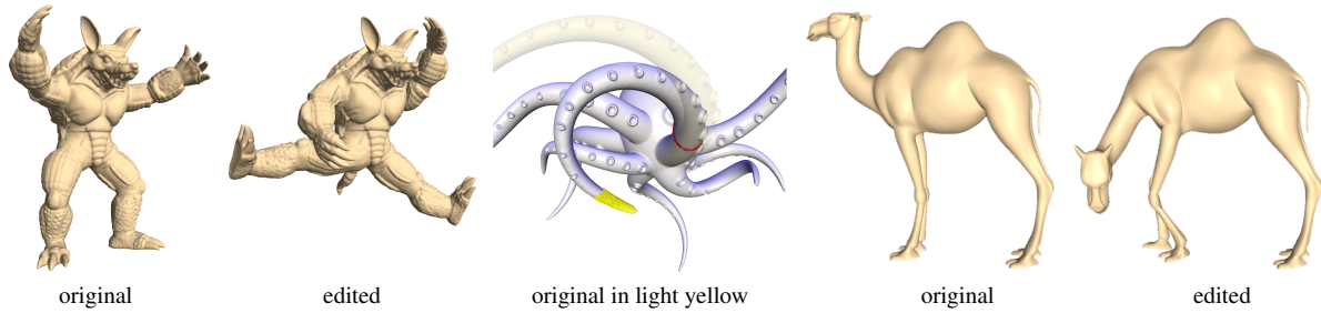
Figure 13: Some editing results using the rotation-invariant representation of [LSLCO05]. Note the large rotational deformations achieved and the preservation of local surface details.
