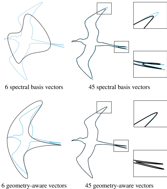
Figure 5: Reconstruction of the swallow curve (simple closed path) using different bases. The top row shows reconstruction using the Laplacian eigenvectors, which are the discrete cosine basis functions in this case. The bottom row displays reconstruction with geometry-aware basis vectors. The reconstructed mesh is shown in black, while the original mesh is tinted in blue. The geometry-aware bases better approximate the features of the shape, on a large as well as on a small scale.
