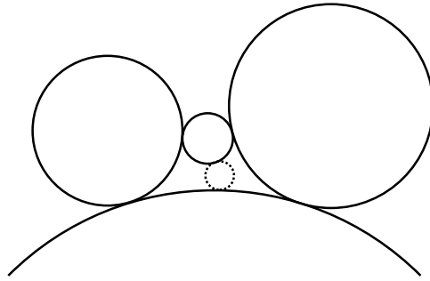
Figure 3. Bad four-sided gap split into two good gaps.
