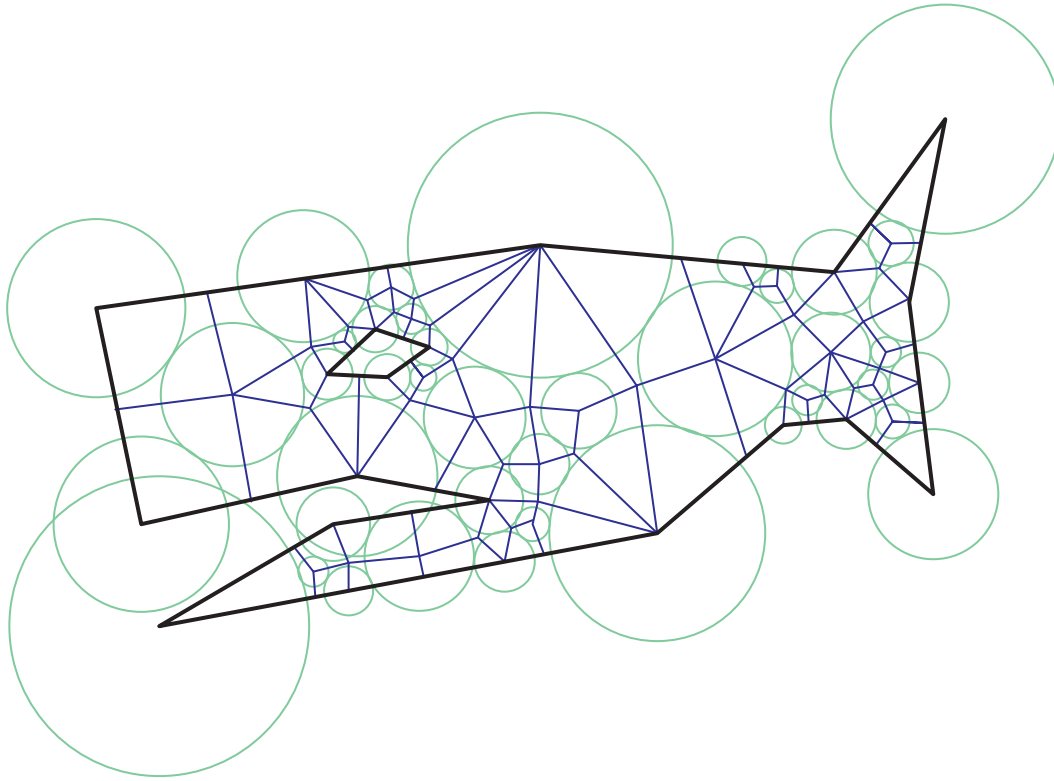
Figure 4. Voronoi quadrilateralization of a polygon.
