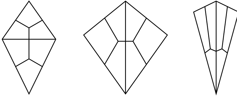
Figure 9. Kites divided into six quadrilaterals with no angle larger than 120^\circ : (a) top and bottom angles both less than 120^\circ ; (b) top and bottom angles both greater than 60^\circ ; (c) top at least 120^\circ and bottom less than 120^\circ .
