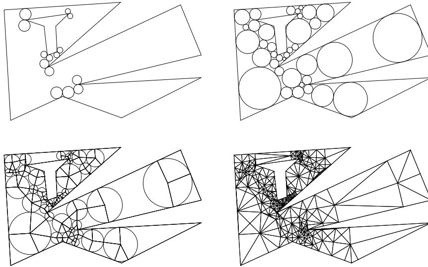
Figure 1. Nonobtuse triangulation steps: (a) protect reflex vertices and connect holes; (b) pack polygon with circles; (c) connect circle centers; (d) triangulate remaining polygonal regions.
