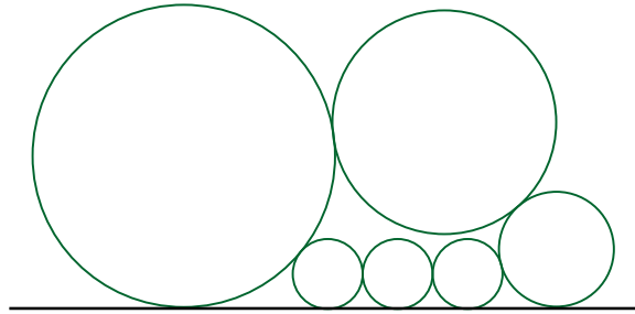
Figure 8. Kite decomposition of four-sided gap with one side on domain boundary: add small circles along boundary edge making three-sided gaps.
