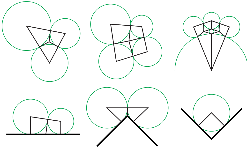
Figure 6. Cases for decomposition into kites: (a) three tangent circles; (b) four tangent circles forming good four-sided gap; (c) bad four-sided gap subdivided into two good four-sided gaps; (d) two tangent circles on boundary; (e) reflex vertex; (f) convex vertex.
