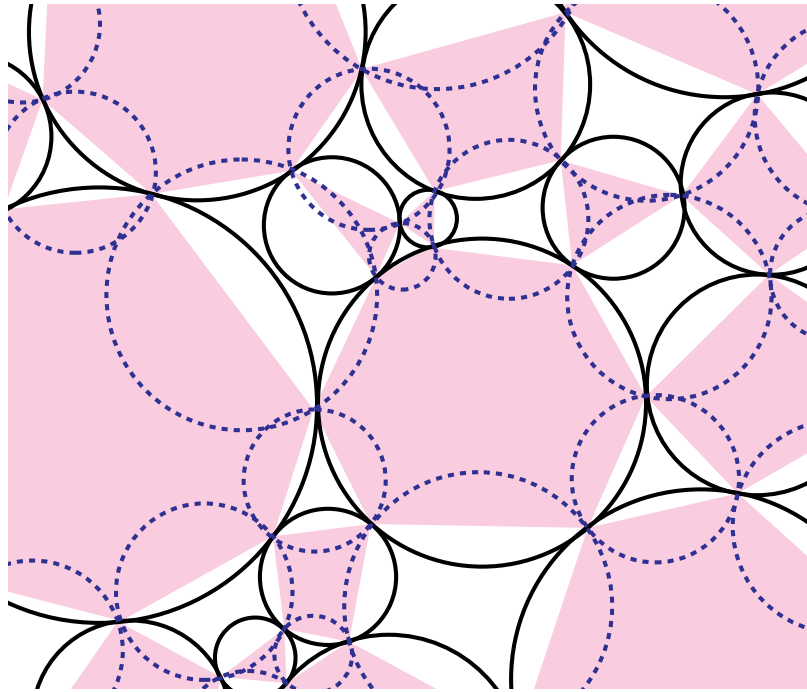
Figure 5. Circle packing (solid circles), circumcircles of gaps (dashed circles), and power diagram (shaded and unshaded polygons).
