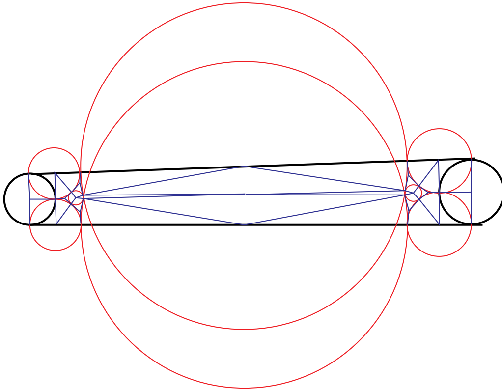
Figure 7. Kite decomposition of four-sided gap with two sides on domain boundary.
