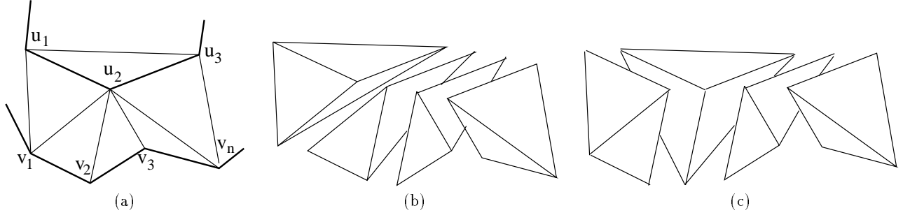
Figure 6: There are different ways to form tetrahedra involving a boundary triangle \Delta u_1 u_2 u_3 .
