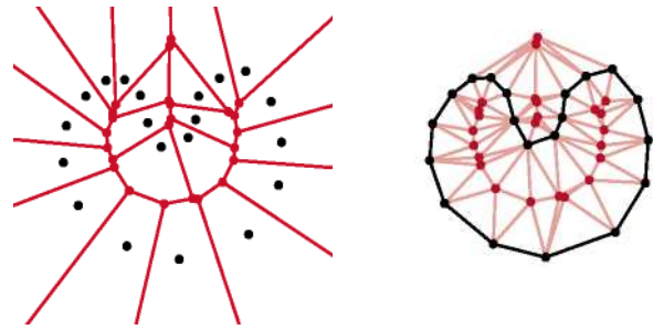
Figure 5. The two-dimensional algorithm. On the left, the Voronoi diagram of a point set S sampled from a curve. Just as S approximates the curve, the Voronoi vertices V approximate the medial axis of the curve. On the right, the the Delaunay triangulation of S \cup V , with the crust edges in black. Theorem 1 states that when S is an r -sample, for sufficiently small r , the crust edges connect only adjacent vertices.
