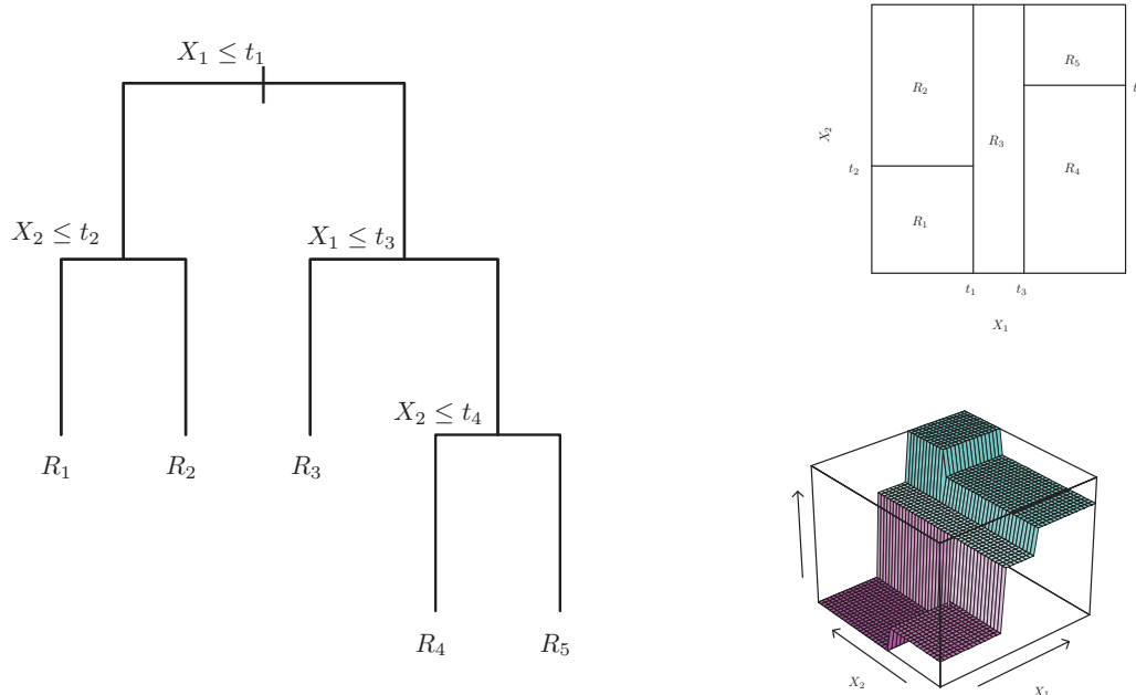
regresstree.pdf, regresstreefn.pdf (ISL, Figure 8.3) [Decision tree regression.]
