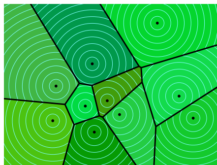
voronoi.pdf [When you have many classes, their LDA decision boundaries form a classical Voronoi diagram if the priors \pi_C are equal. All the Gaussians have the same width.]
