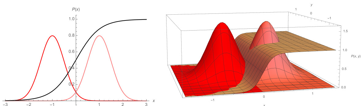
lda1d.pdf , lda2d.pdf [Two Gaussians (red) and the logistic function (black). The logistic function is the right Gaussian divided by the sum of the Gaussians. Observe that even when the Gaussians are 2D, the logistic function still looks 1D.]
