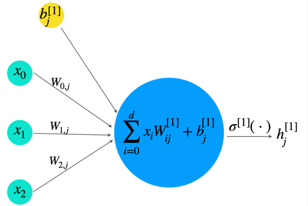
Figure 2: A single fully-connected neuron.
