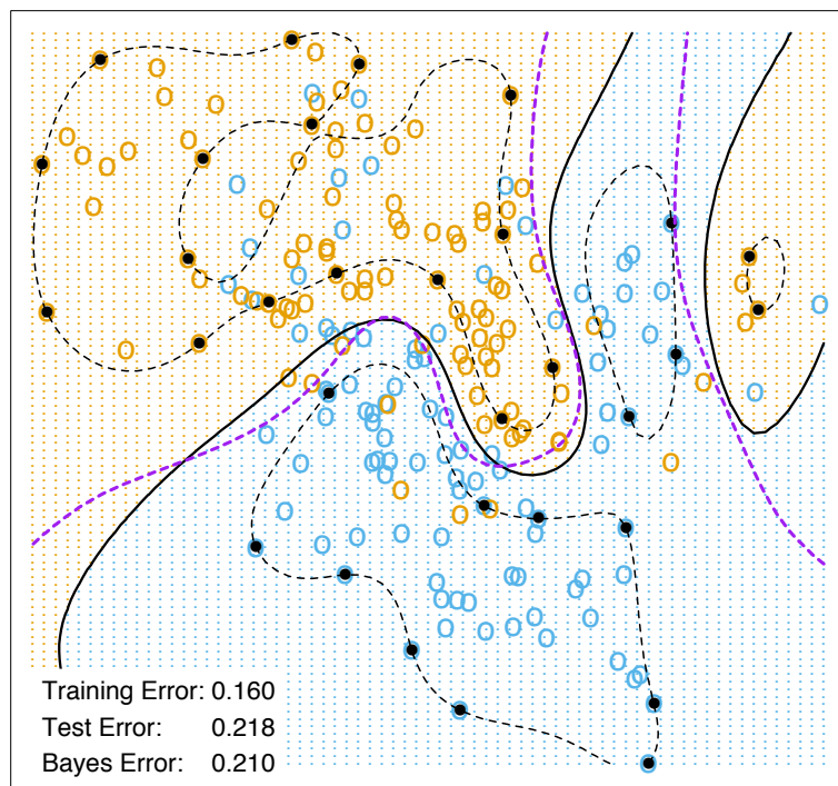
gausskernelsvm.pdf (ESL, Figure 12.3) [The decision boundary (solid black) of an SVM with a Gaussian kernel. Observe that in this example, it comes reasonably close to the Bayes optimal decision boundary (dashed purple).]
