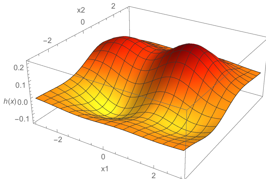
gausskernel.pdf [A hypothesis h that is a linear combination of Gaussians centered at four sample points, two with positive weights and two with negative weights.]
