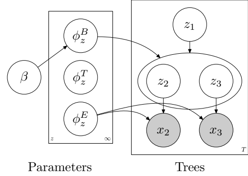
Figure 2: The definition and graphical model of the HDP-PCFG. Since parse trees have unknown structure, there is no convenient way of representing them in the visual language of traditional graphical models. Instead, we show a simple fixed example tree. Node 1 has two children, 2 and 3, each of which has one observed terminal child. We use L(i) and R(i) to denote the left and right children of node i .
