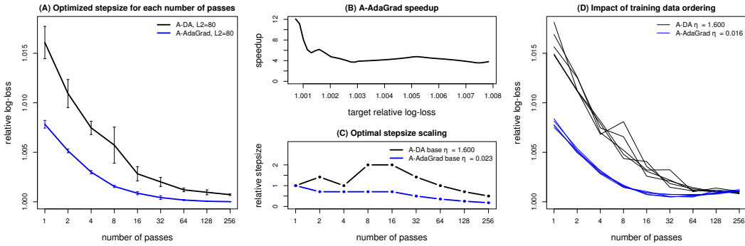
Figure 3. (A) Relative test-set log-loss for ASYNCDADA and ASYNCDADAGRAD, choosing the best stepsize (within a factor of about 1.4\times ) individually for each number of passes. (B) Effective speedup for ASYNCDADAGRAD. (C) The best stepsize \eta , expressed as a scaling factor on the stepsize used for one pass. (D) Five runs with different random seeds for each algorithm (with \ell_2 penalty 80).
