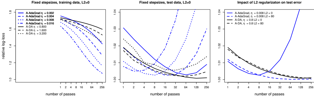
Figure 2: Relative accuracy for various stepsize choices on a click-through rate prediction dataset.
