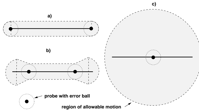
Figure 4: Relationship of placement of probes (solid points) with error balls (dashed circles) along an edge (solid line) and the resulting displacement region (shaded). (a) Probes at endpoints of edge. (b) Probes moved inward from edge resulting in larger region of allowable motion. (c) Probes coincident at center of edge, allowing maximum displacement region.
