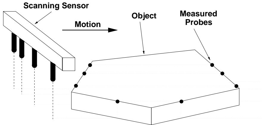
Figure 3: Example of a fixed array scanning beam sensor
