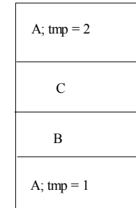
Execution stack
