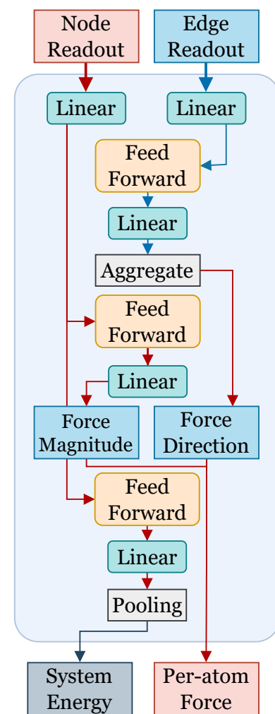
(c) Output Block
