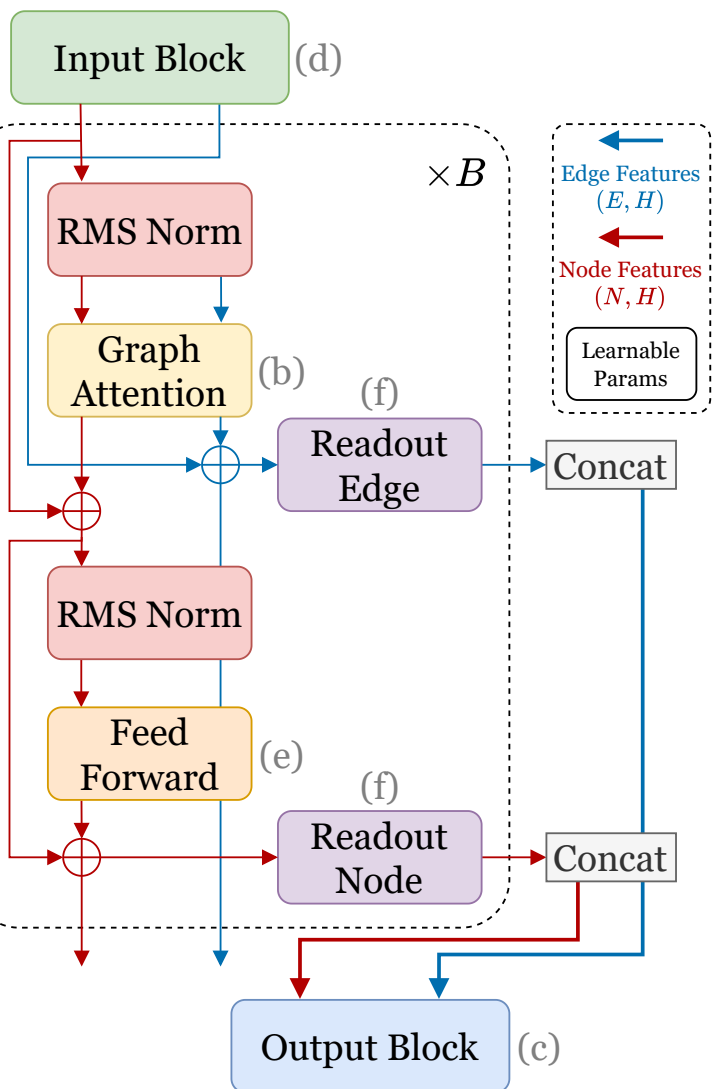
(a) EScAIP Architecture
