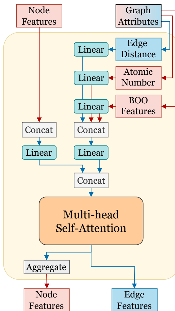
(b) Graph Attention
