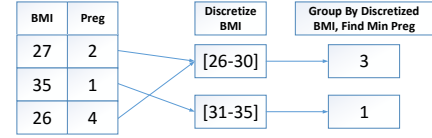
Fig. 2: An illustrations of the operators used by ExploreKit in the generation of a feature in the Pima dataset
