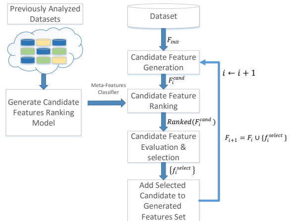
Fig. 1: ExploreKit system architecture
