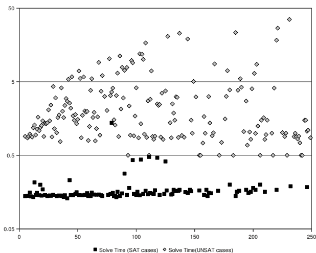
Figure 13: The constraint solver’s running time (in seconds) as a function of the size of the input constraints (in terms of the number of symbolic JavaScript operations)
